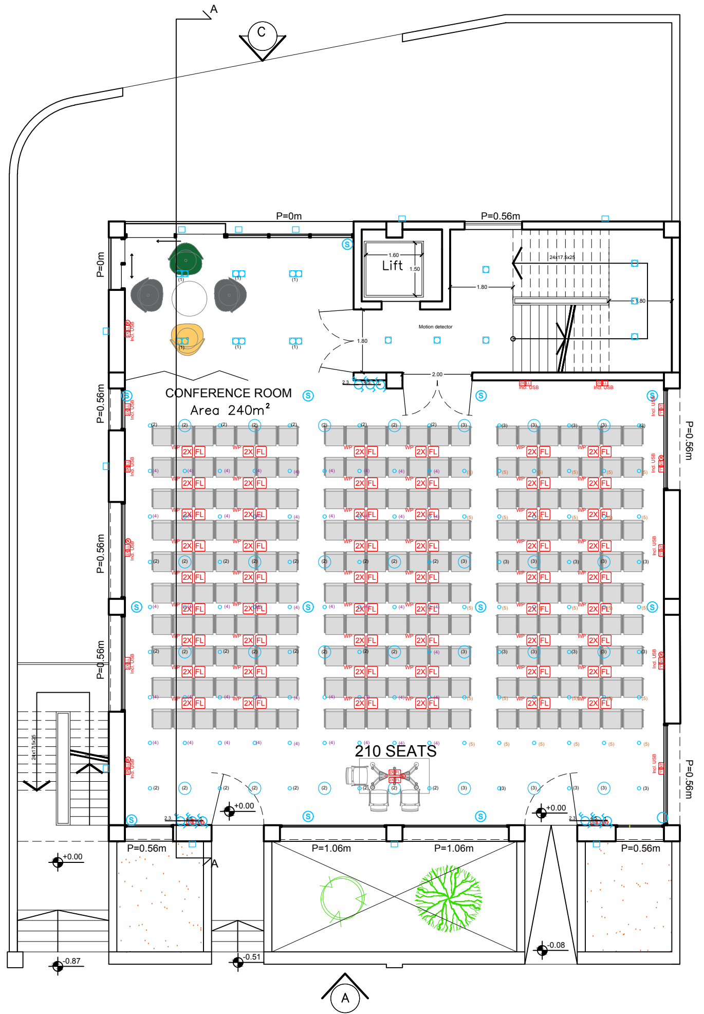
PROPOSED LEVEL 0 PLAN SCALE 1:100
